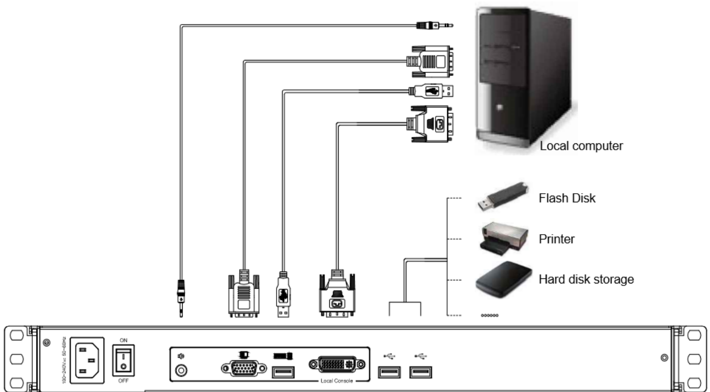
KVM-2401WPD-REAR-COVER
