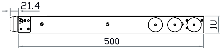
Side View
