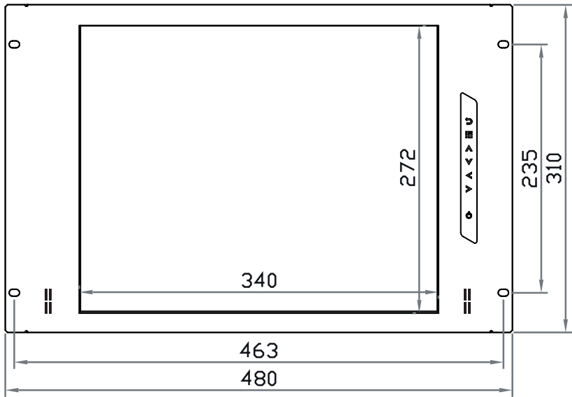
Front View RMPH-161-17
