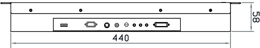
Bottom View
